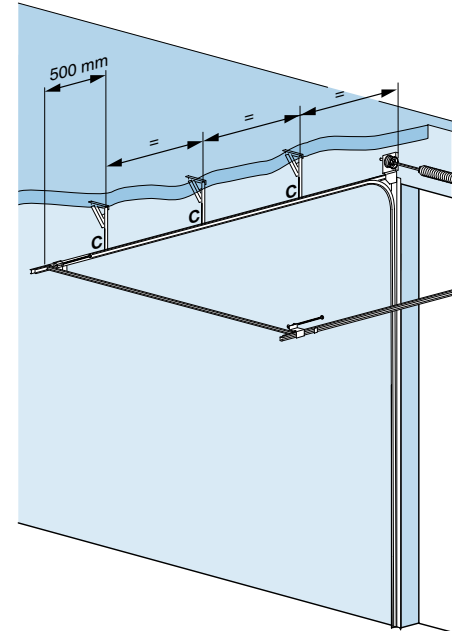
C: LH > 5000 mm
