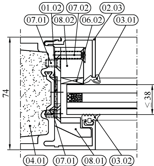
Scheibe "CONTRAFLAM 30"
